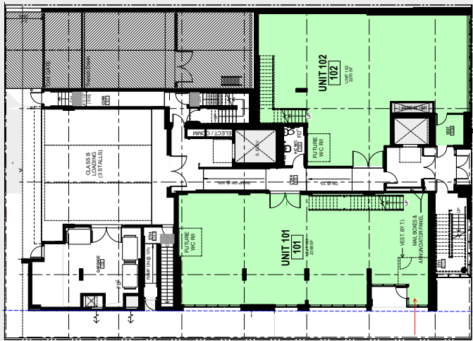
LEVEL 1 PLAN UNIT 101: 2,398 SF MAIN FLOOR + 1,428 SF MEZZANINE UNIT 102: 2,270 SF MAIN FLOOR + 1,796 SF MEZZANINE
